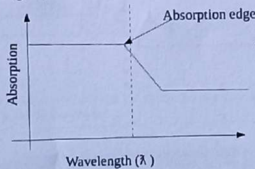
Fig: Variation of absorption of light by Semiconductor with its wavelength.
