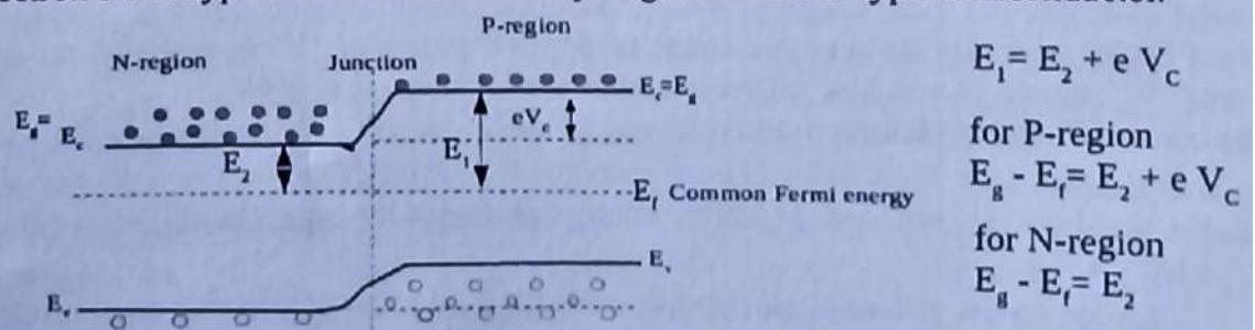
Fig: Energy band after contact of N-type and P-type semiconductor.
